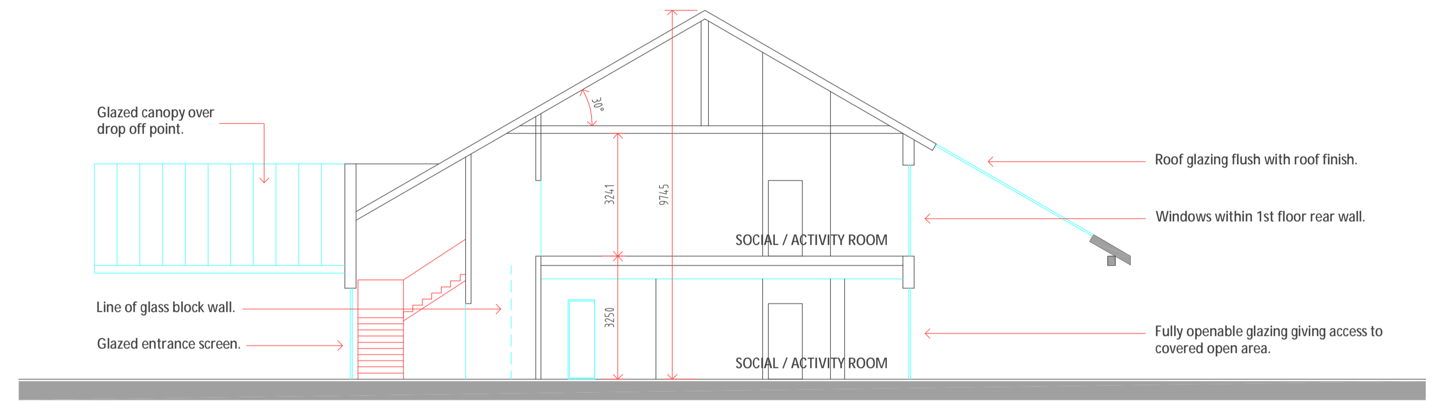
SECTION THRO' MAIN BUILDING
